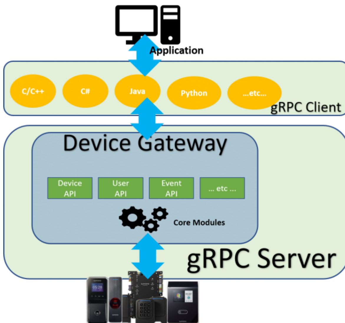
[Figure 1. G-SDK architecture]
